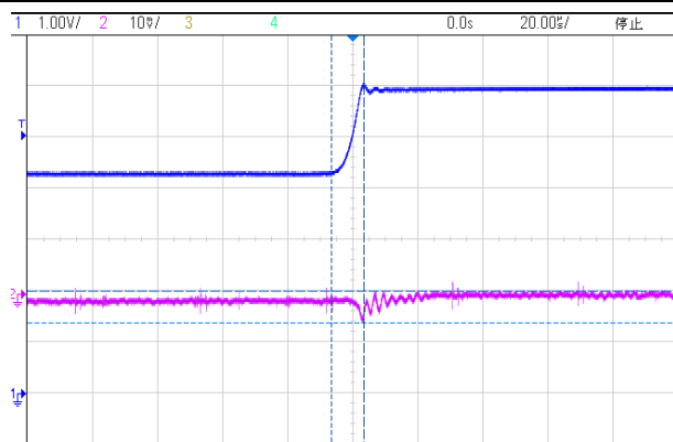
Input Transient(4.3~6V t=10us 10mA)
