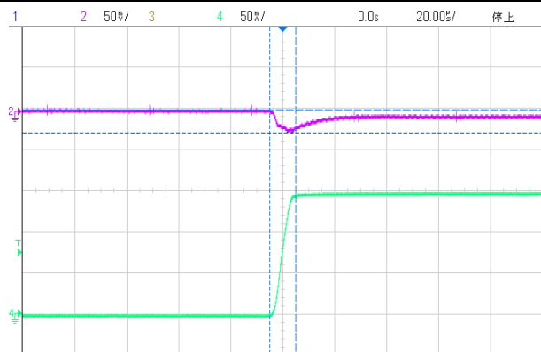
Load Transient(1mA~150mA t=10us)
