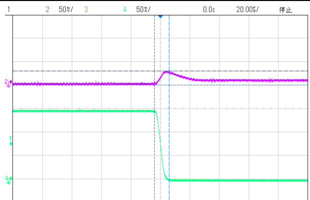
Load Transient(150mA~1mA t=10us)
