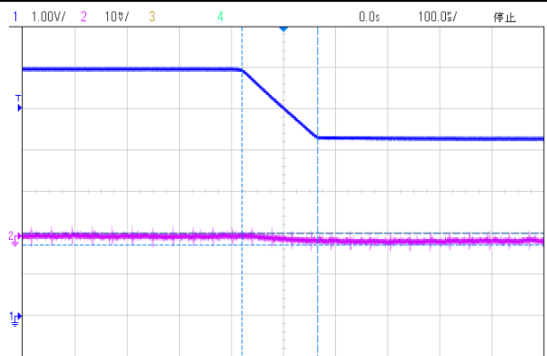
Input Transient(6~4.3V t=10us 10mA)
