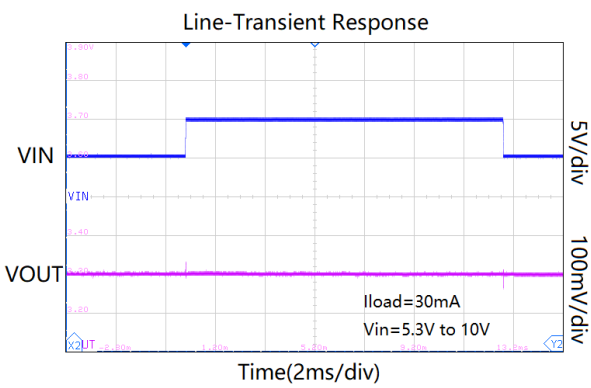
Line-Transient Response
