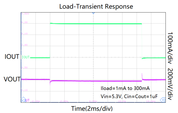
Load-Transient Response
