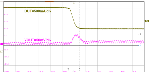
10us/div, V_{OUT}=3.3V I_{OUT} = 3A to 1.5A Figure32. ET81311 Load Transient
