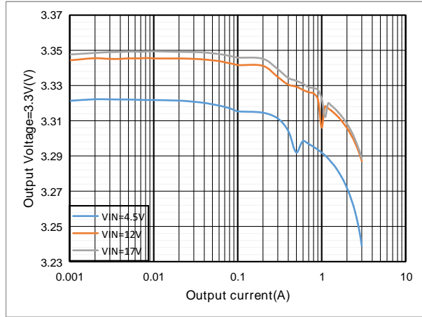
Figure12. ET81311 Load Regulation, V_{OUT}=3.3V
