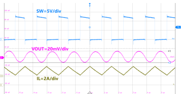
1us/div, V_{OUT}=5.0V I_{OUT}=3A Figure28. ET81311 Output Ripple
