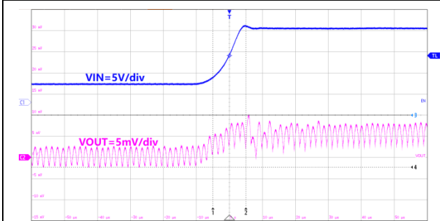
10us/div, V_{OUT}=1.0V I_{OUT} = 1.5A V_{IN}=4.5V to 17V Figure35. ET81311 Line Transient
