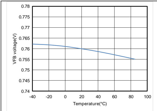
Figure5. ET81311 VFB Voltage vs Temperature
