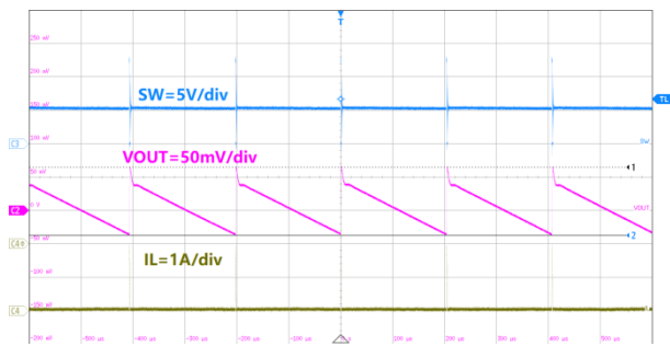
100us/div, V_{OUT}=5.0V I_{OUT}=10mA Figure25. ET81311 Output Ripple
