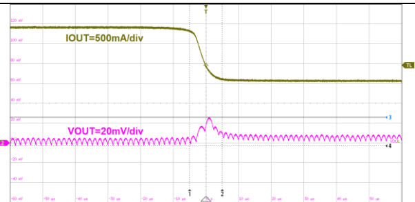
10us/div, V_{OUT}=1.0V I_{OUT} = 3A to 1.5A Figure30. ET81311 Load Transient
