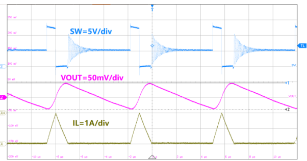
2us/div, V_{OUT}=5.0V I_{OUT}=250mA Figure26. ET81311 Output Ripple
