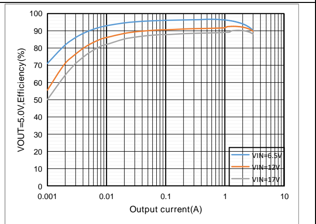
Figure8. ET81311 Efficiency vs Output Current
