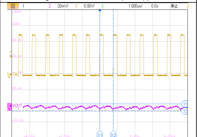
1us/div, V_{OUT}=3.3V I_{OUT} = 500mA Figure20. ET81313 Output Ripple
