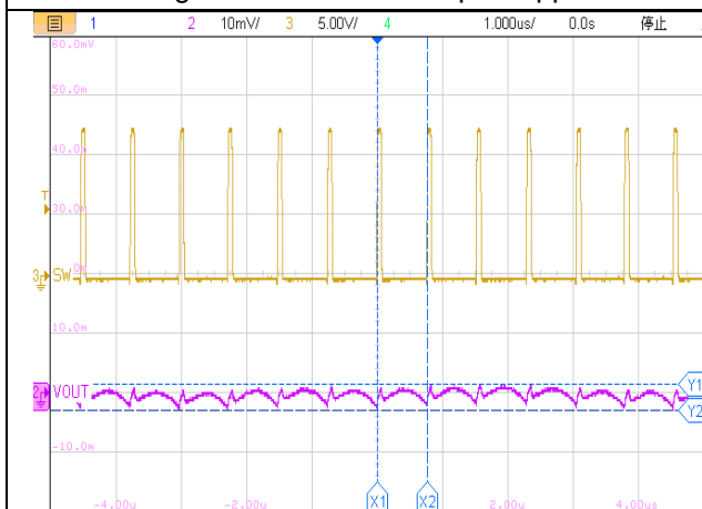
1us/div, V_{OUT}=1.0V I_{OUT}=1.5A Figure17. ET81313 Output Ripple
