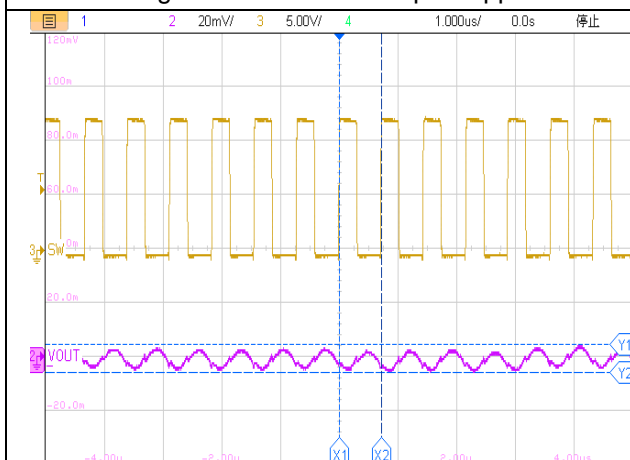
Figure23. ET81313 Output Ripple
