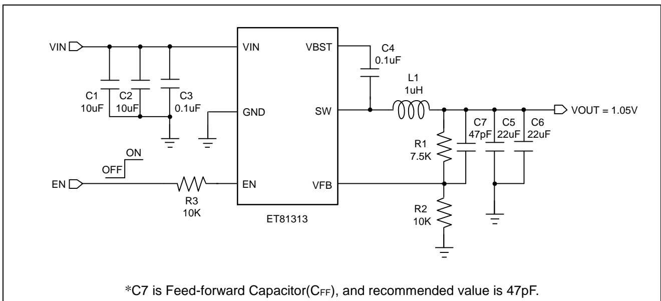
V_{OUT}=1.05V/3A Reference Design
