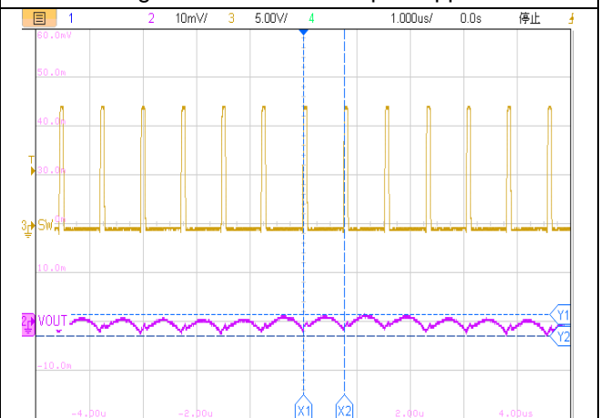
1us/div, V_{OUT}=1V I_{OUT}=3A Figure18. ET81313 Output Ripple
