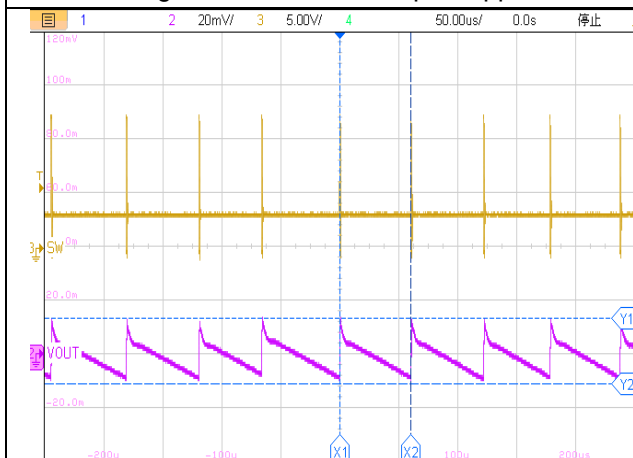
50us/div, V_{OUT}=3.3V I_{OUT} = 10mA Figure19. ET81313 Output Ripple
