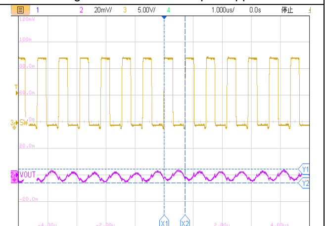
Figure22. ET81313 Output Ripple
