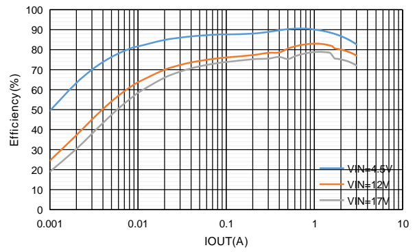
Figure6. ET81313 Efficiency vs Output Current
