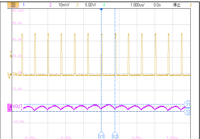
1us/div, V_{OUT}=1.0V I_{OUT} = 500mA Figure16. ET81313 Output Ripple
