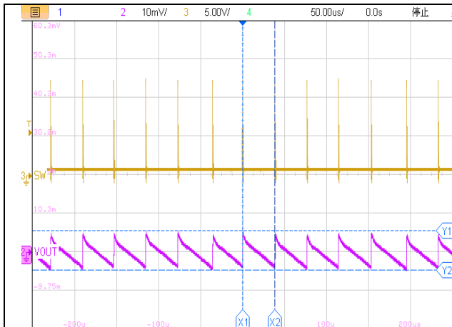
50us/div, V_{OUT}=1.0V I_{OUT} = 10mA Figure15. ET81313 Output Ripple
