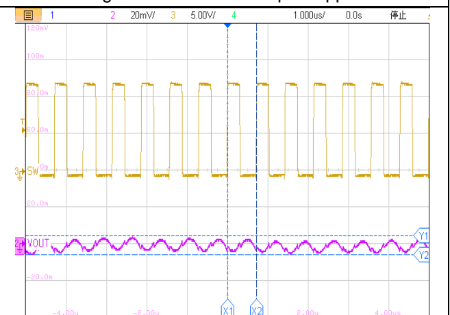
Figure24. ET81313 Output Ripple
