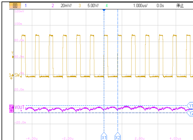
Figure21. ET81313 Output Ripple
