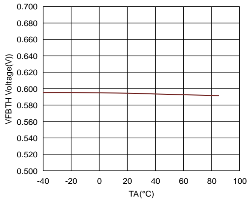
Figure5. ET81313 V_{FB} Voltage vs Temperature
