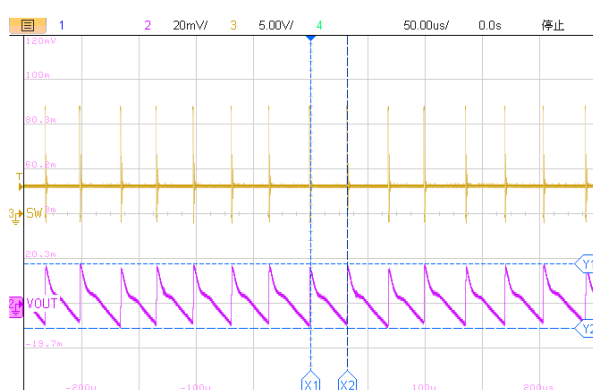
50us/div, V_{OUT}=3.3V I_{OUT}=10mA Figure19. ET81413 Output Ripple
