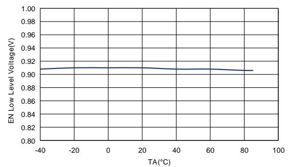
Figure4. ET81413 EN_L vs Temperature
