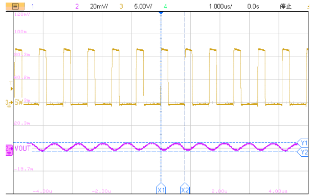
1us/div, V_{OUT}=3.3V I_{OUT}=4A Figure22. ET81413 Output Ripple
