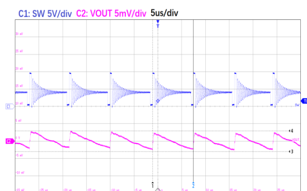
Figure13. ET84501 Output Ripple
