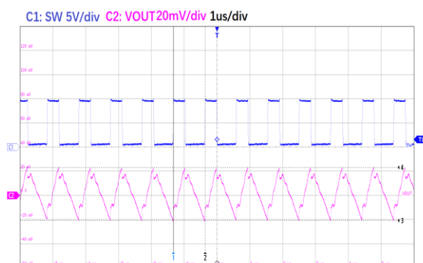
Figure15. ET84501 Output Ripple
