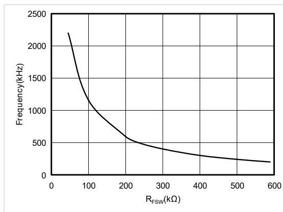
Figure8. ET84501 Switching Frequency Setting
