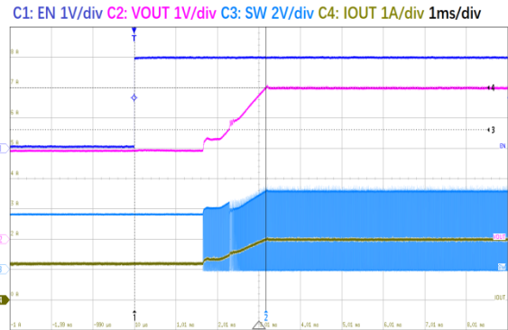
Figure20. ET84501 Start-Up to EN
