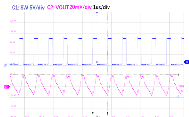
Figure16. ET84501 Output Ripple
