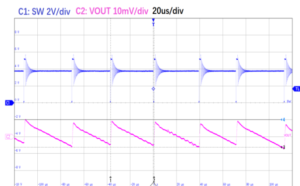
Figure10. ET84501 Output Ripple
