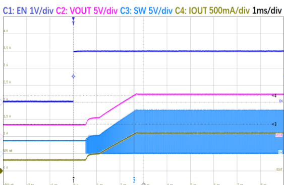
Figure22. ET84501 Start-Up to EN
