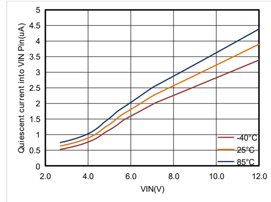
Figure3. ET84501 Quiescent current into VIN Pin
