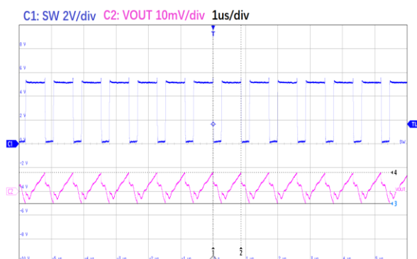
Figure12. ET84501 Output Ripple
