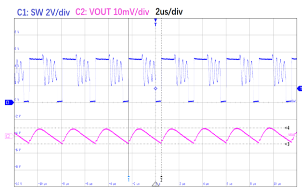
Figure11. ET84501 Output Ripple
