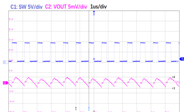
Figure14. ET84501 Output Ripple
