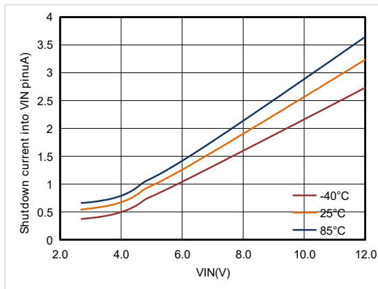
Figure4. ET84501 Shutdown current into VIN pin
