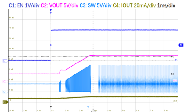
Figure21. ET84501 Start-Up to EN
