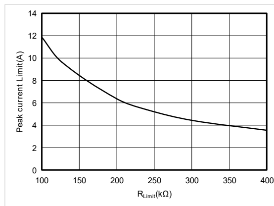
Figure9. ET84501 Switching Peak Current Limit Setting
