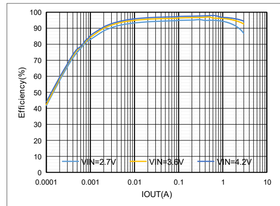
Figure5. ET84501 Efficiency vs Output Current
