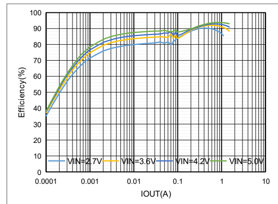
Figure7. ET84501 Efficiency vs Output Current
