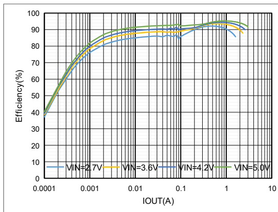
Figure6. ET84501 Efficiency vs Output Current
