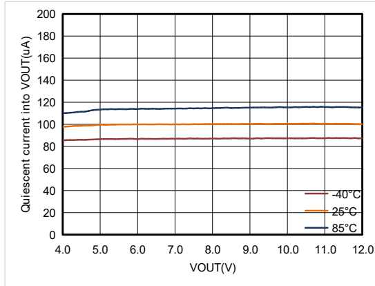
Figure2. ET84501 Quiescent current Into VOUT Pin
